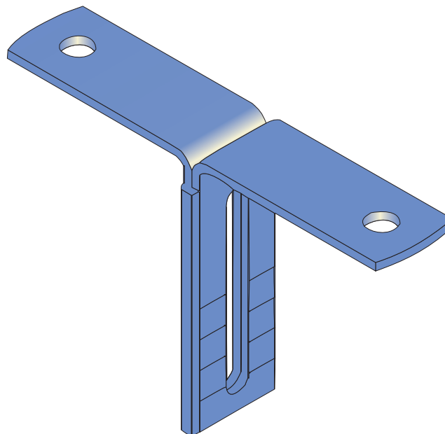
FM117 ADJUSTABLE STAND-OFF BRACKET FINISH: ZINC PLATED
