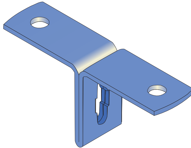
FM116 STANDARD STAND-OFF BRACKET FINISH: ZINC PLATED
